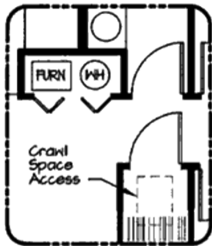
Crawl Space / Slab Plan
